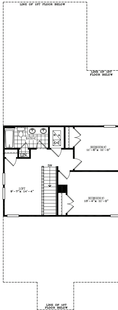
SECOND FLOOR PLAN ELEVATION "A"
