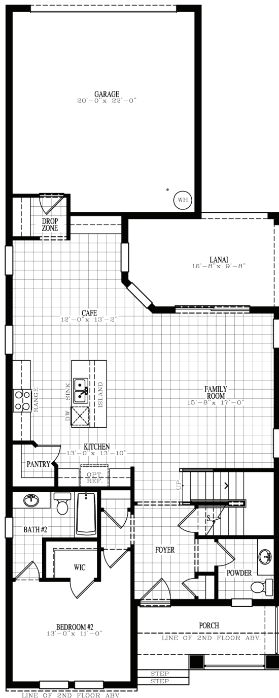
FIRST FLOOR PLAN ELEVATION "A"
