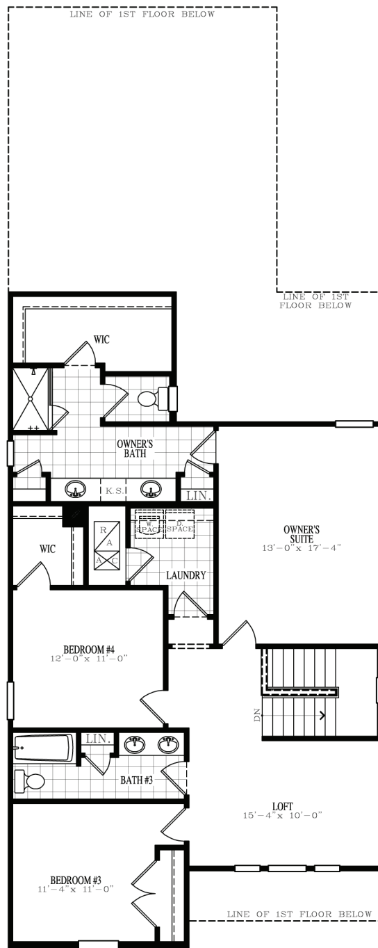
SECOND FLOOR PLAN ELEVATION "A"
